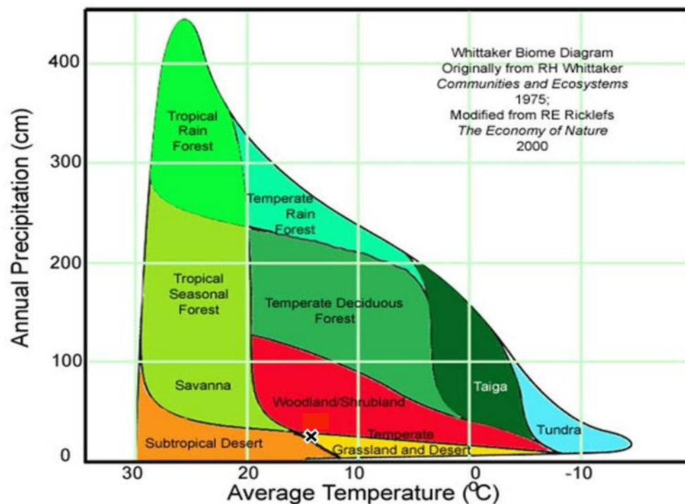
Figure 10. Whittaker Biome Diagram
