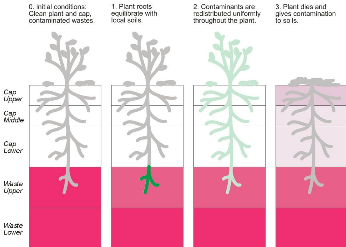
Figure 9. Conceptual model for plant induced contaminant transport
