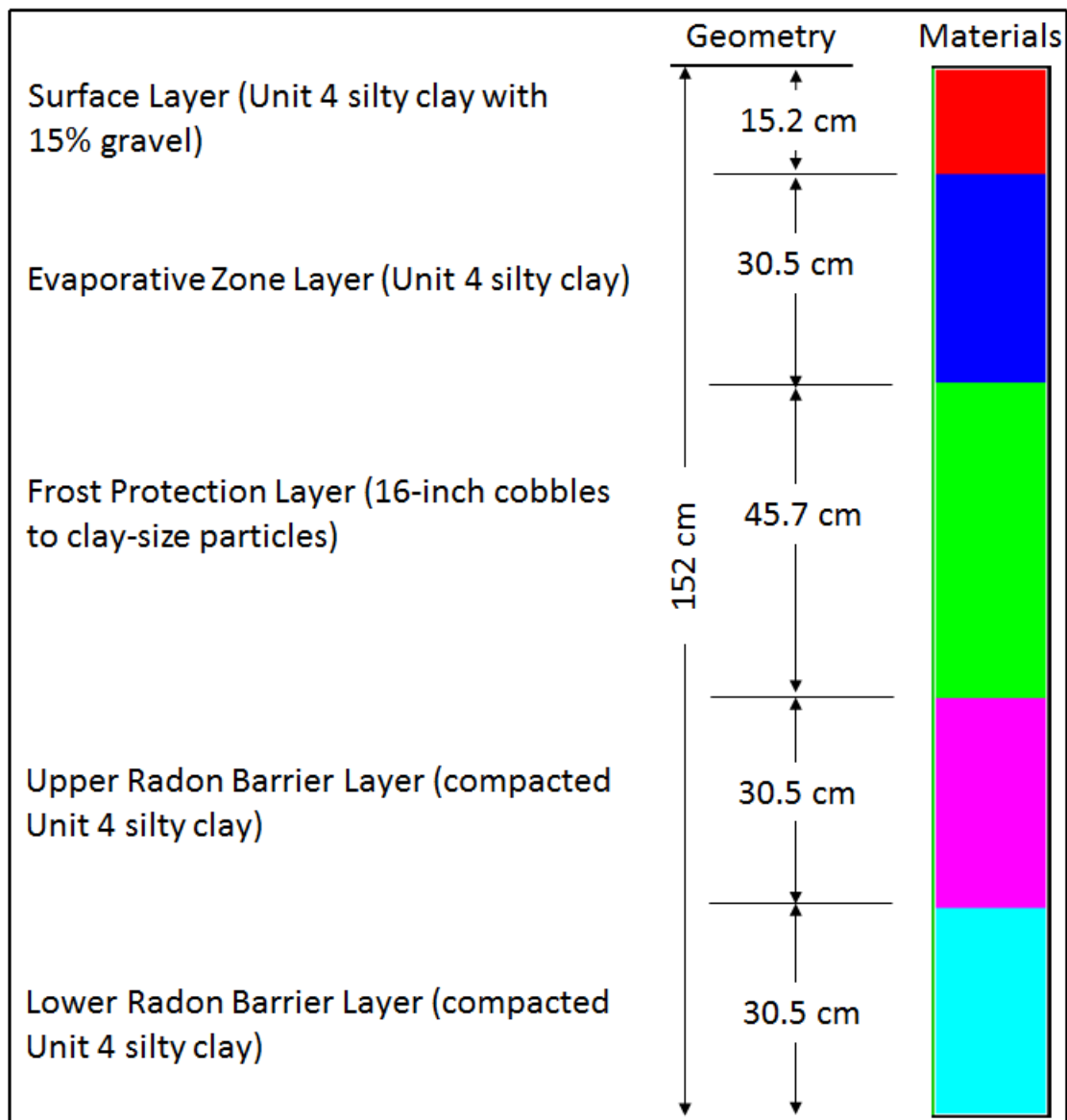
Figure 7. Evapotranspiration (ET) cover system.
