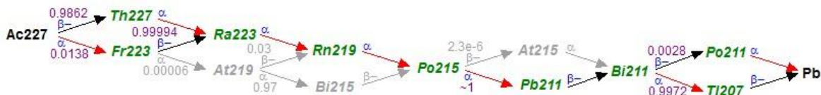
Figure 13. Detailed decay chains for actinides. Radionuclides in black are included in the fate and transport model, those in green are considered only in the dose model, and those in gray are not modeled.
